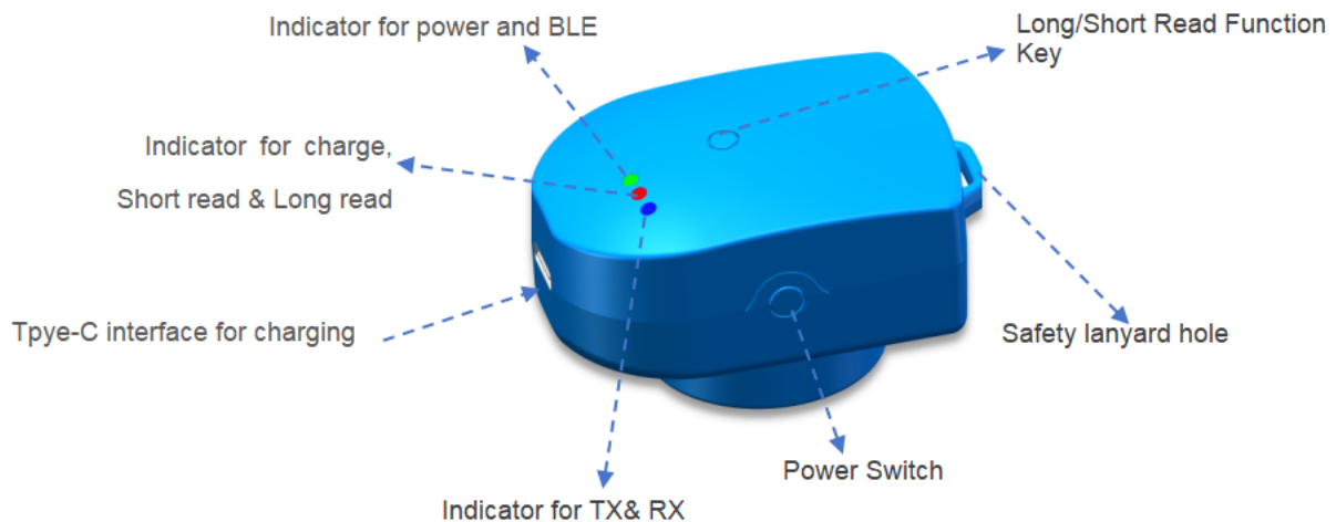
Fig.3 Component descriptions
